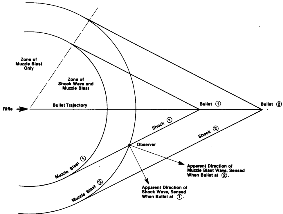
FIG. 1. LOCI OF MUZZLE BLAST AND SHOCK WAVES AT TWO TIMES AFTER FIRING OF BULLET.
