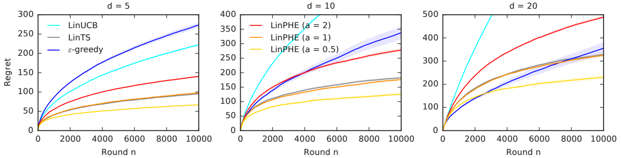
Figure 1: Comparison of LinPHE to several baselines in three linear bandit problems. All results are averaged over 100 random problem instances. The shaded areas are standard errors of the estimates. The legend is split between the first two plots.
