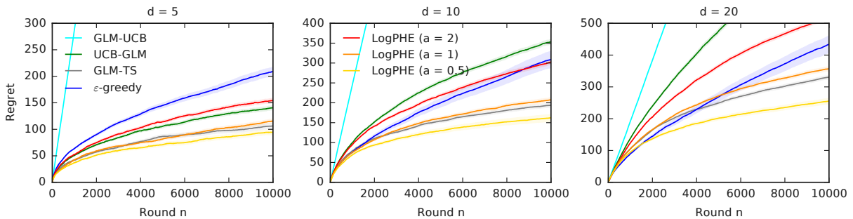
Figure 2: Comparison of LogPHE to several baselines in three logistic bandit problems. All results are averaged over 100 random problem instances. The shaded areas are standard errors of the estimates. The legend is split between the first two plots.
