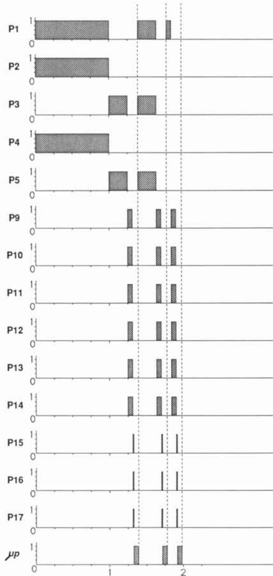
Figure 7. Time utilization for three iterations of the coarse-fine, focal, motion analysis procedure.
