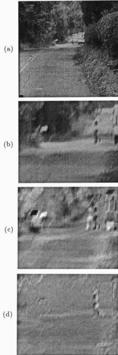
Figure 2. (a) Postman crossing road. (b) Region selected for motion analysis. (c) Difference between successive image frames showing motion due to the camera and postmen. (d) Difference after detecting and compensating for surface motion within the analysis region.
