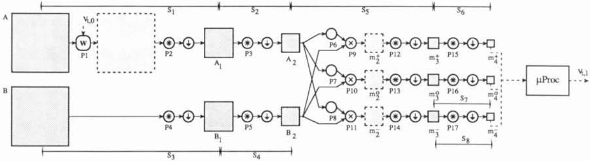
Figure 6. Motion computation diagram.
