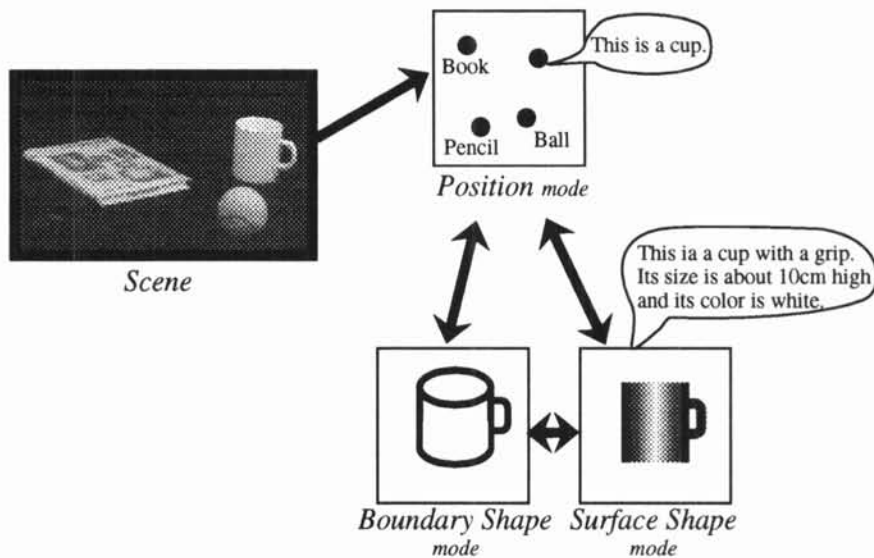
Figure 7: Interactive interface.
