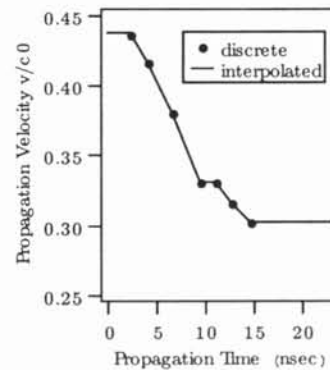
Figure 6: Estimated propagation velocity distribution v(t) .
