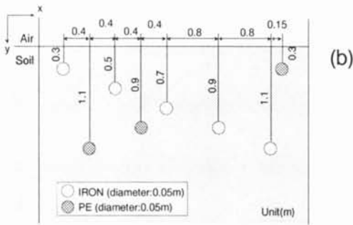
Figure 4: Subsurface radar image and its cross-section. (a) subsurface radar image obtained by impulse-radar; (b) cross-section.
