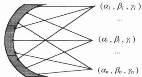
Figure 5. Single arc statistic recognition with triplets.
