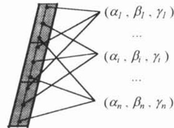
Figure 3. Single straight line recognition with triplets.
