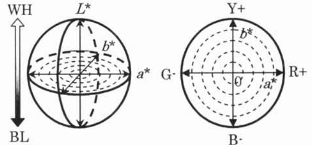
Figure 1: L^*a^*b^* Color System
