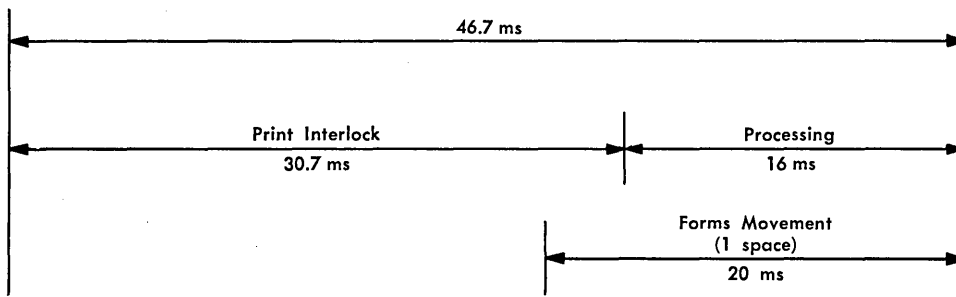
Figure 232. Print Timing Chart (Numerical)
