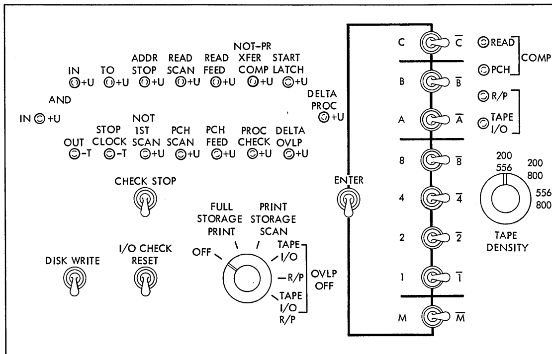
Figure 196. Auxiliary Console
