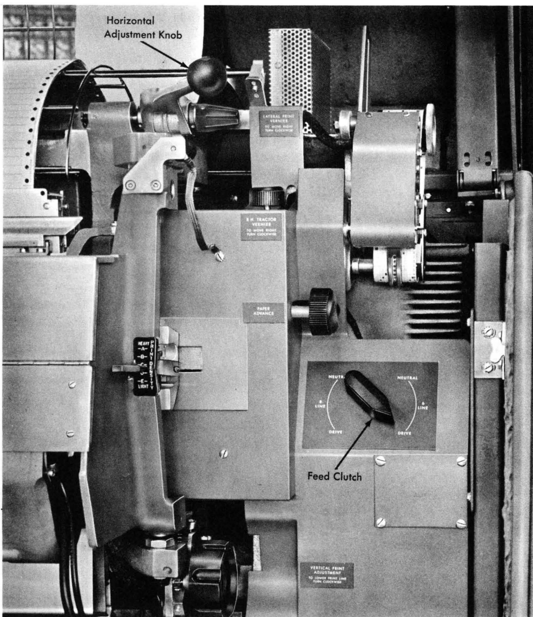
Figure 200. Manual Controls
