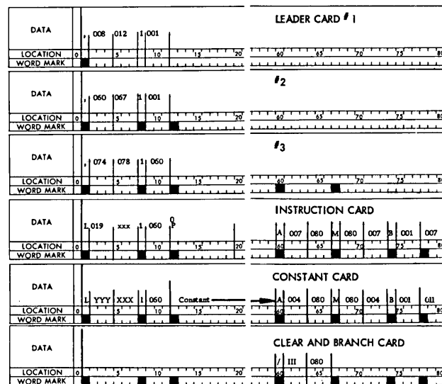
Figure 259. Instruction Cards
