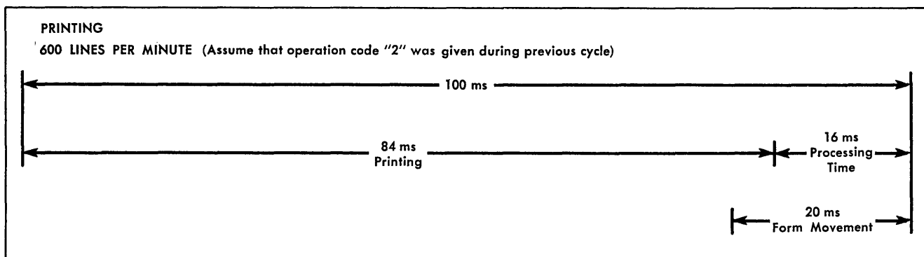
Figure 67. Print Cycle
