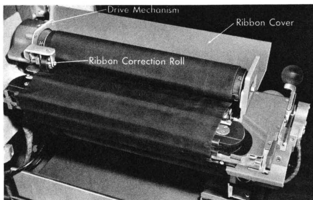
Figure 208. Ribbon Mechanism
