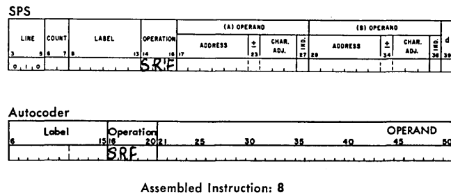
Figure 141. Read Release
