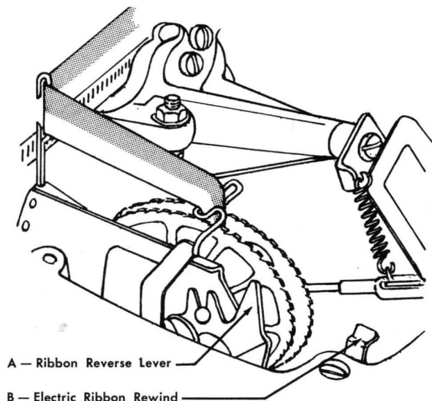
Figure 217. Ribbon Reverse
