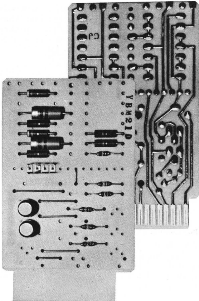
Figure 2. Transistor Cards
