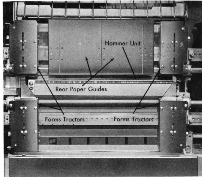
Figure 211. Forms Tractor
