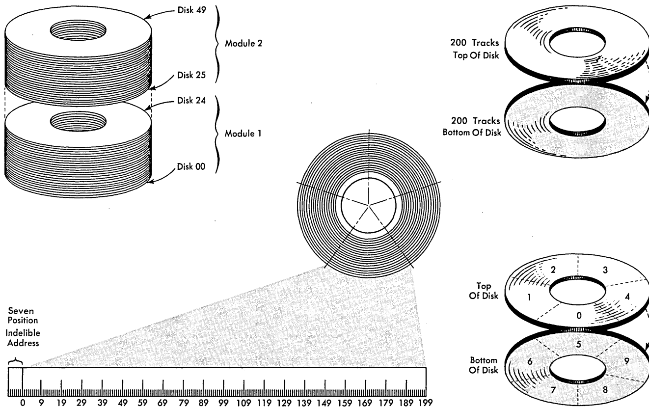
Figure 110. Disk Storage
