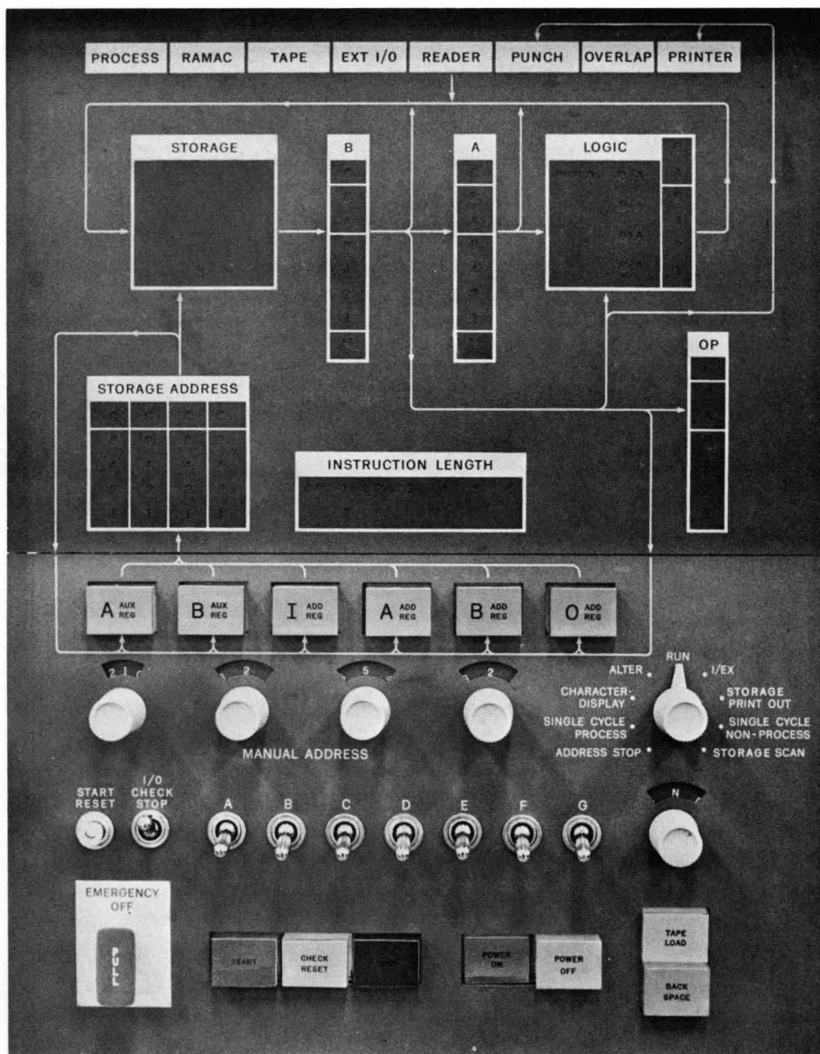
Figure 195. IBM 1401 Console
