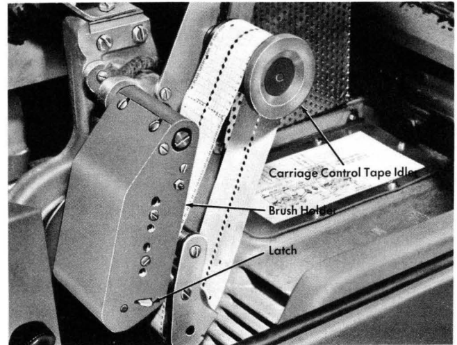
Figure 205. Tape-Controlled Carriage
