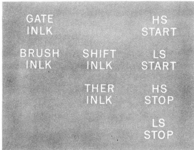
Figure 204. Printer Indicator Panel
