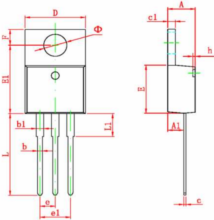
TO-220F
