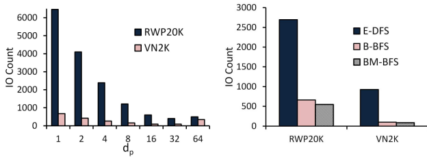
Figure 12: IO count vs different partition depths
