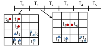
Figure 2: ReachGrid Index Example
