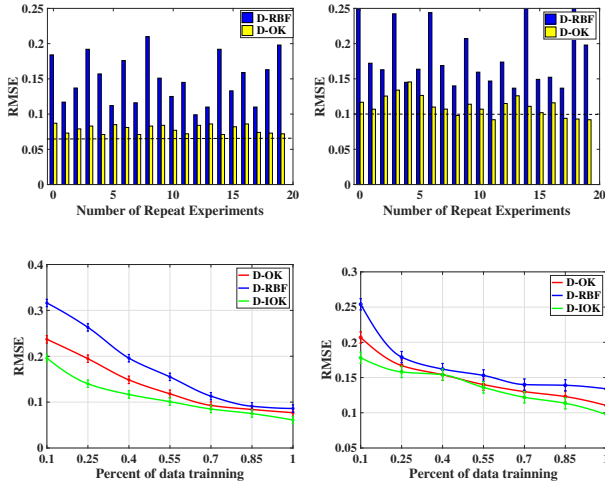
Figure 3: From left to right. Top : The stability test between D-OK and D-RBF for synthetic data set generated from F_1(\mathbf{x}) and F_2(\mathbf{x}) respectively; Bottom : The test RMSE versus decreasing percent of training data generated from F_1(\mathbf{x}) and F_5(\mathbf{x}) respectively.
