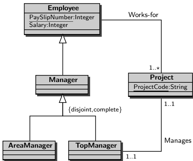
Figure 2: The UML diagram used as example.
