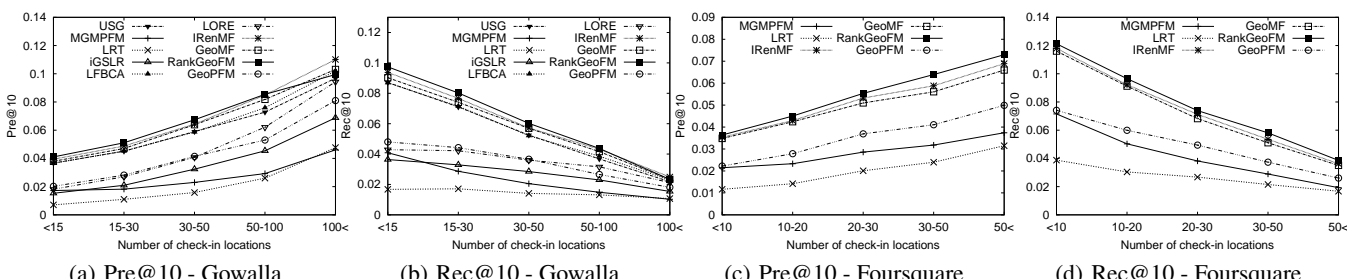
Figure 6: Performance of POI recommendations for users with different numbers of check-in POIs
