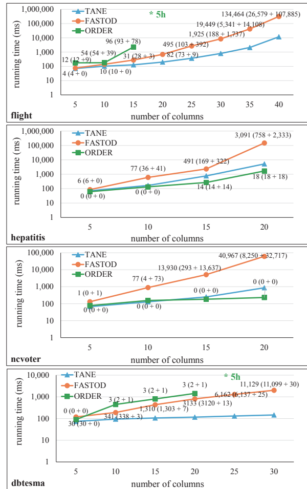
Figure 7: Scalability and effectiveness in |R| .
