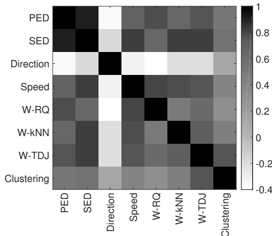
Figure 5: Correlation analysis of the error metrics.
