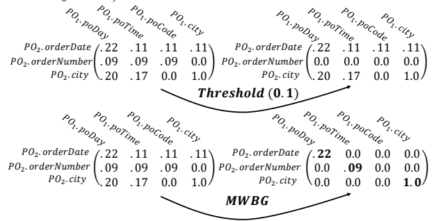
Figure 4: Similarity matrix adjustment example
