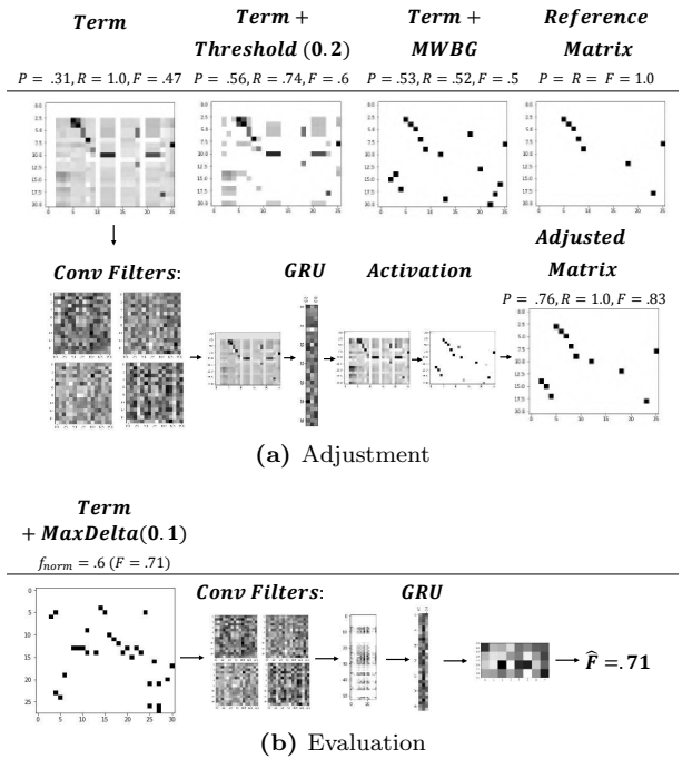
Figure 6: AD and EV illustration over Web-forms pairs (Section 4.1). Entries are marked by a gray scale color map. 4
