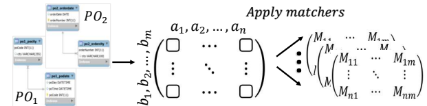
Figure 2: Similarity matrix generation
