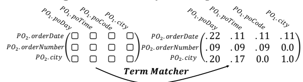
Figure 2: Similarity matrix generation
