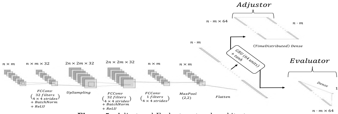
Figure 5: Adjust and Evaluate network architecture.
