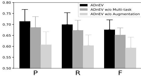
Figure 11: Effect of Multi-task Learning and Augmentation on ADnEV’s performance: (P)recision , (R)ecall, (F)1
