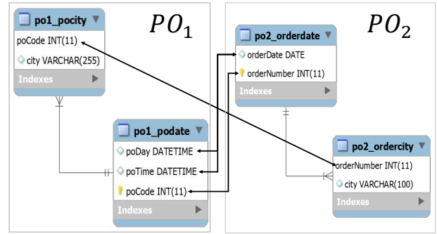
Figure 1: Schema Matching example
