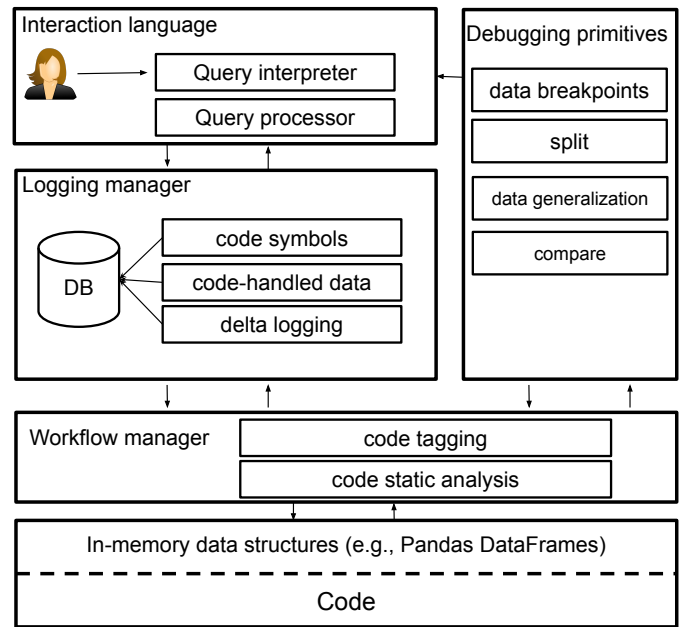
Figure 1: Dagger architecture
