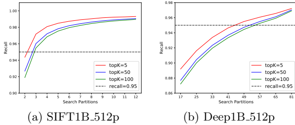
Figure 11: Performance analysis for clustering-based partition pruning.
