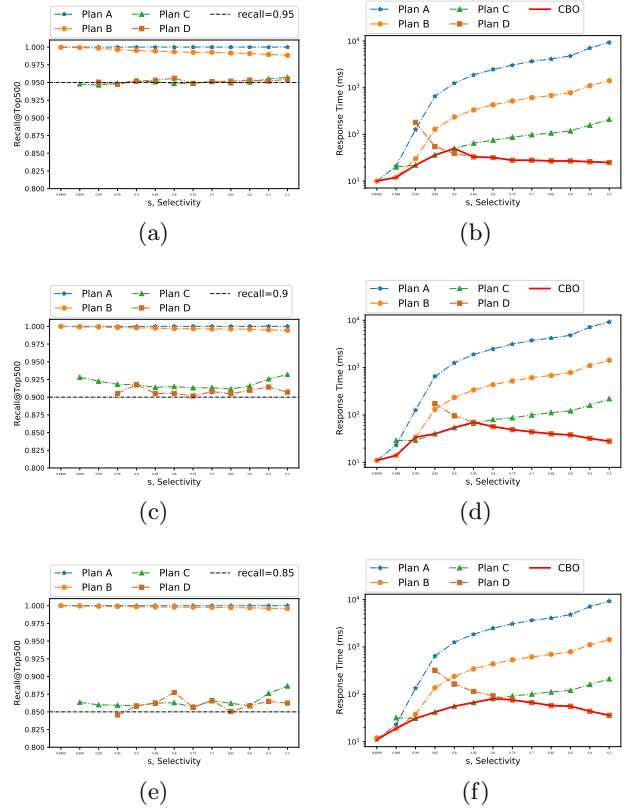
Figure 12: Performance study of different physical plans.
