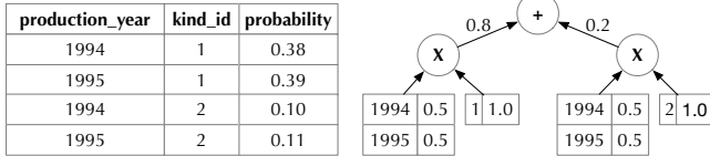
Figure 5: An example of Sum Product Network.
