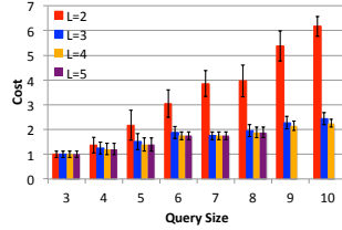
Figure 18: Relaxation cost vs query size, for CDR-L (Homes dataset).
