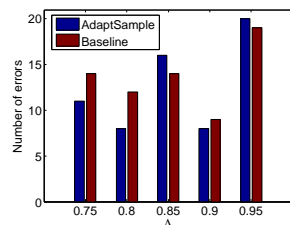
(f) Number of errors w.r.t. query threshold \Lambda
