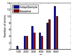
(b) Number of errors w.r.t. number of objects m
