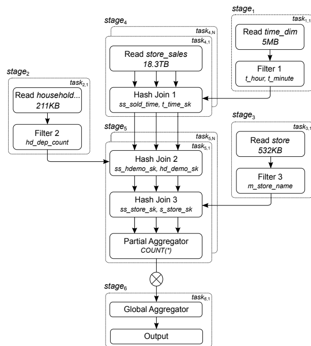
Figure 3: An Execution Plan for TPC-DS Query 96.
