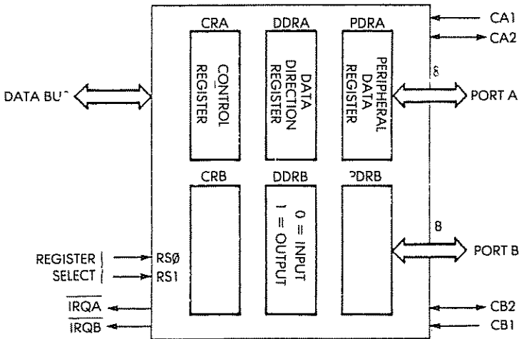
Fig. 7.1: Typical PIO
