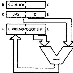
Fig. 3.31: 16/8 Division—The Registers
