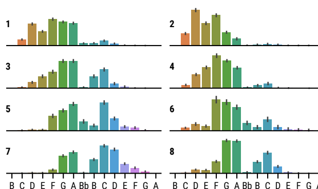
Figure 3. Pitch profiles showing the relative frequency of every pitch in each of the 8 modes. Again, although the distribution of individual modes are clearly distinct, some residual ambiguity remains.
