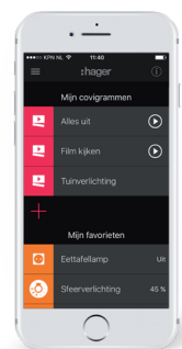
Covigrammen
