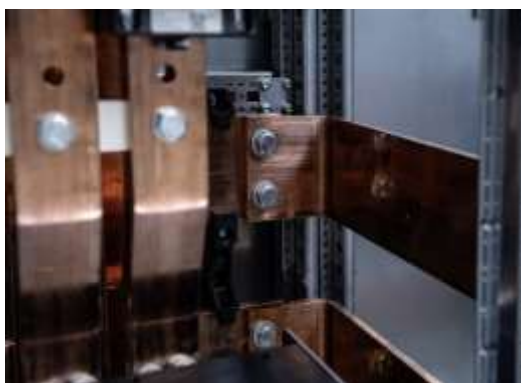
Detail kast-kastverbinding
