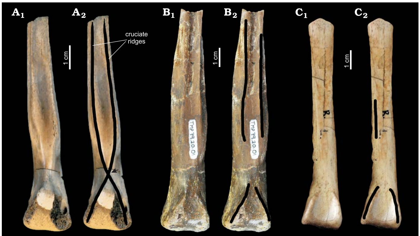
Fig. 4. Posterior surface of metatarsal III in elmisaurine dinosaurs. A. Leptorhynchus elegans (Parks, 1933) (TMP 1986.036.0186) from Upper Campanian Dinosaur Park Formation, Dinosaur Provincial Park, Alberta, Canada. B. Chirostenotes pergracilis Gilmore, 1924 (TMP 1979.020.0001) from Upper Campanian Dinosaur Park Formation, Dinosaur Provincial Park, Alberta, Canada. C. Ingenia yanshini Barsbold, 1981 (MPC-D 102/011), provenance unknown: confiscated specimen. Photographs (A 1 –C 1 ), annotated photographs (A 2 –C 2 ), black lines indicate longitudinal ridges; arrow indicates cruciate ridge feature of Leptorhynchus elegans .
