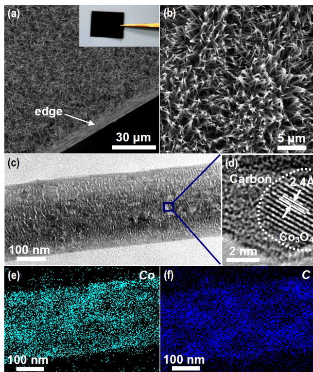
Figure 1. (a, b) SEM, (inset in panel a) optical image, (c) TEM, (d) HRTEM, and (e, f) EDS elemental mapping images of \text{Co}_3\text{O}_4\text{C-NA} .
