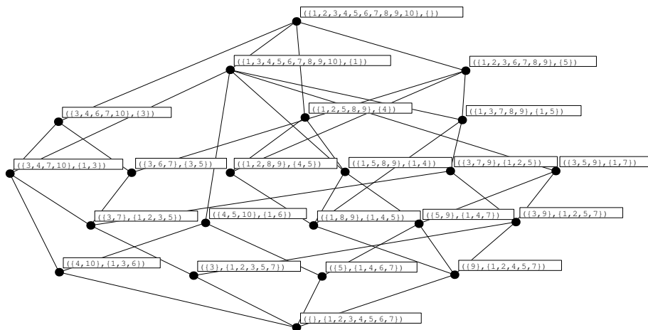
Fig. 3. Concept lattice corresponding to the context from Tab. 2
