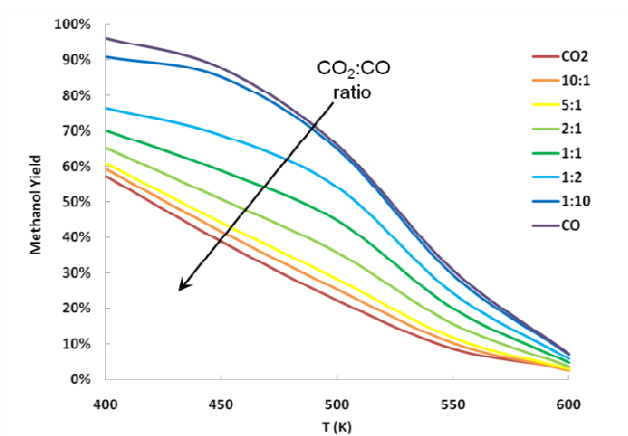
Figure 7. Equilibrium yield of methanol at 50 bar from 3:1 CO 2 /CO/H 2 mixtures as a function of CO 2 /CO ratio
