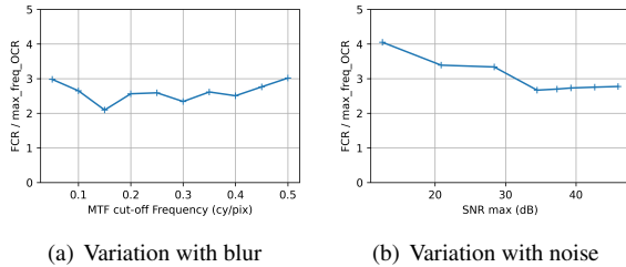
Figure 18. Maximum resolved frequency for OCR and FCR, for different blur and noise levels
