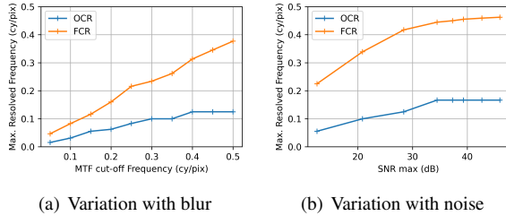
Figure 17. Maximum resolved frequency for OCR and FCR, for different blur and noise levels
