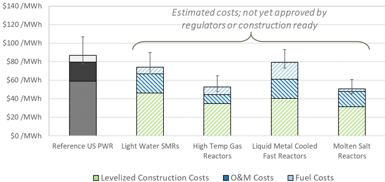
Figure 10. LCOE for SMRs and Advanced Reactor Technologies
