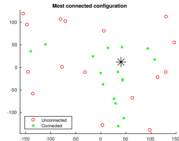
Fig. 9: The most connected configuration (50.00% connected) of a Poisson point process with density \lambda = 0.001 and \tau = -60 (or \tau_\lambda = -30 ) dB.
