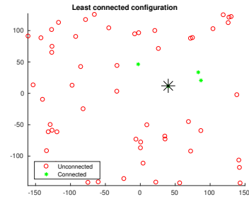
Fig. 8: The least connected configuration (7.02% connected) of a Poisson point process with density \lambda = 0.001 and \tau = -60 (or \tau_\lambda = -30 ) dB.
