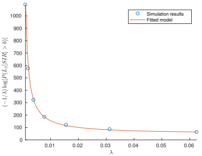
Fig. 6: Simulation estimate of -\log \mathbb{P}(L_\lambda[\text{SIR}] > b)/\lambda with \tau = -50 dB and \epsilon = 0.05 , fitted to a model \hat{y}_2 = -p_1 - p_2/\lambda , p_1 = -46.65 and p_2 = -1.077 .
