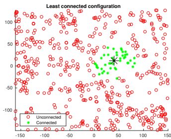
Fig. 10: The least connected configuration (17.99% connected) of a Poisson point process with density \lambda = 0.01 and \tau = -60 (or \tau_\lambda = -40 ) dB.
