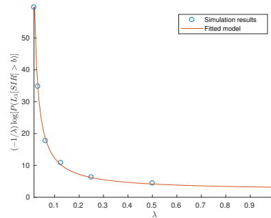
Fig. 4: Simulation estimate of -\log \mathbb{P}(L_\lambda[\text{SIR}] > b)/\lambda with \tau = -50 dB and \epsilon = 0.01 , fitted to a model \hat{y}_2 = p_1 + p_2/\lambda , where p_1 = -2.138 and p_2 = -1.014 .
