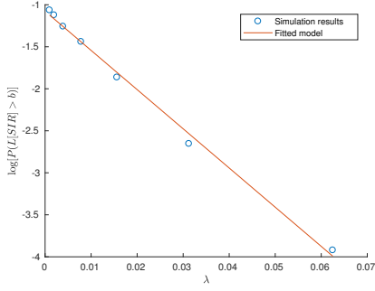
Fig. 5: Simulation estimate of \log \mathbb{P}(L_\lambda[\text{SIR}] > b) with \tau = -50 dB and \epsilon = 0.05 , fitted to a linear model \hat{y}_1 = p_1\lambda + p_2 , where p_1 = -46.65 and p_2 = -1.077 . The value of -p_1 is an estimate for the rate function.
