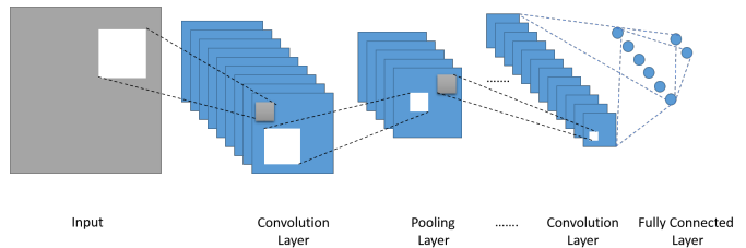
Fig. 2. Different parts of a CNN
