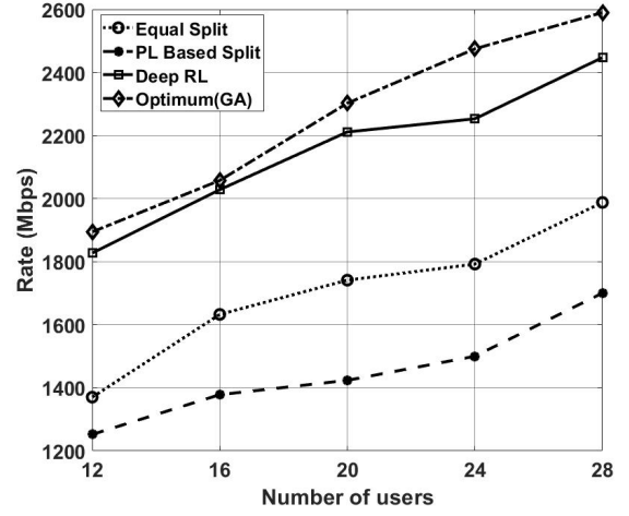
Fig. 6. Total rate versus different number of users
