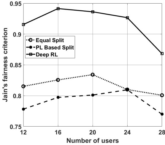
Fig. 8. Jain's fairness criterion
