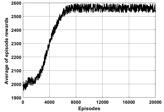
Fig. 5. Average reward of training the agent
