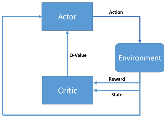
Fig. 3. Actor-critic model
