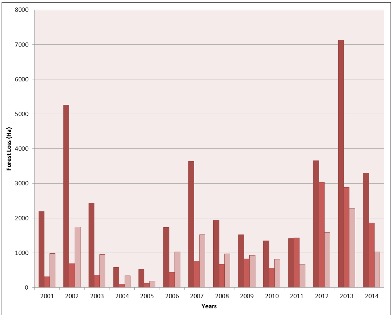
Figure 3.29 Regional Deforestation, 2001–2014
