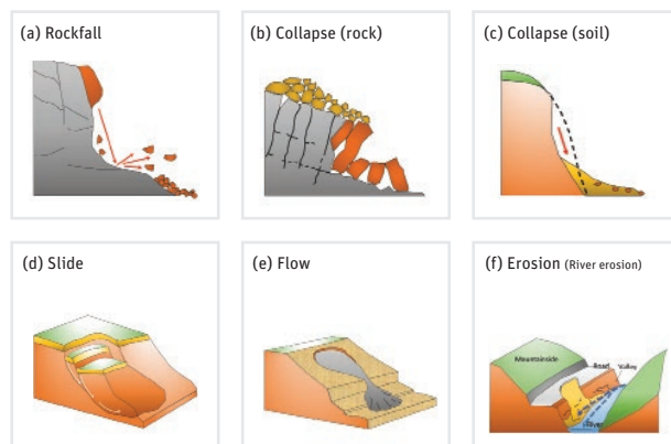
Figure 1: Classification of Geohazards for Roads
