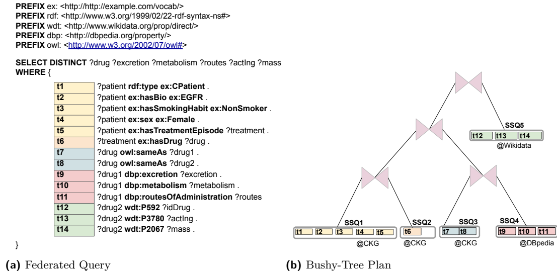
Figure 10 Federated query. a) SPARQL query comprising 14 triple patterns to be executed over a federation including Cancer Knowledge Graph (CKG), DBpedia, and Wikidata. b) A query plan composed of five star-shaped subqueries SSQ1, SSQ2, SSQ3, SSQ4, and SSQ5 corresponding to the query decomposition. Each SSQ is executed over the graph that can answer the SSQ. The execution engine follows the query plan; the execution of four joins merges the SSQ answers and produces the federated query answer.
