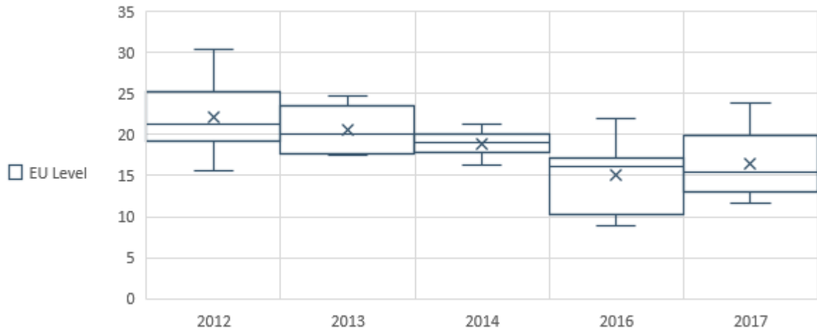
Figure 4. Electricity costs of BOF steel production (€/tonne)
