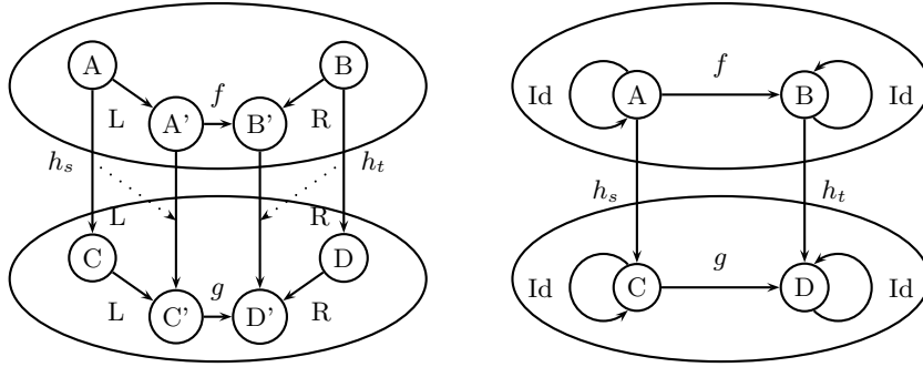
Figure 2: Two comma objects and a comma arrow (h_s, h_t) between them: (left) in general, and (right) for the topos. The rectangles in the middle must commute.
