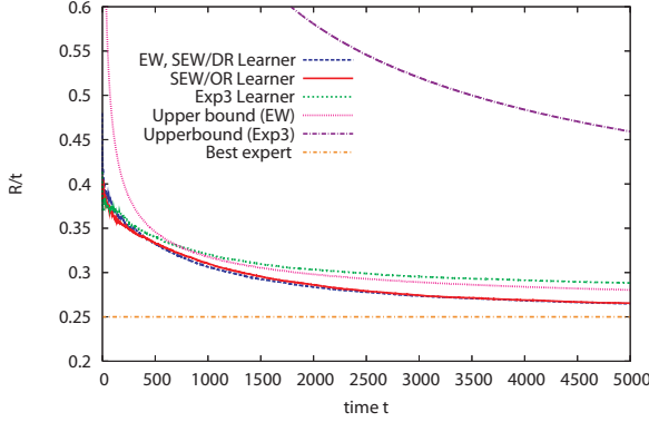
Figure 3. Expectation of regret per time (avg. of 100 iterations, N = 10 , T = 5000 ).
