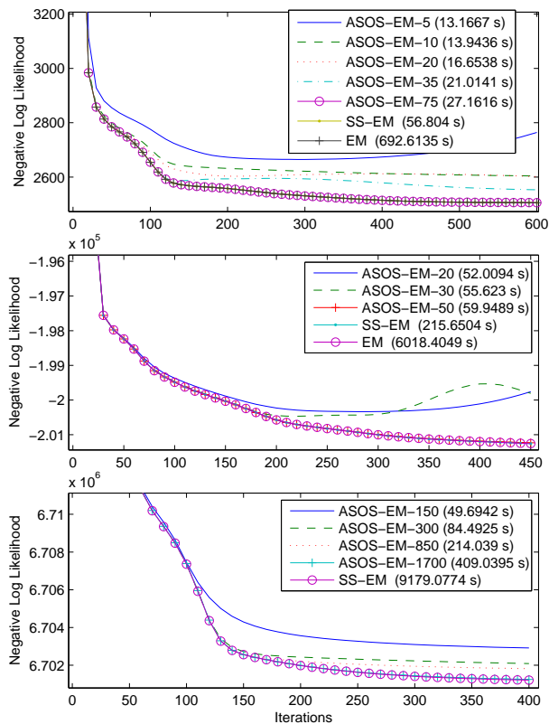
Figure 1. NOTE: Running times are included in the figure legends in brackets. Top: Results from the evaporator dataset with N_x = 15 . Middle: Results from the mo-cap data with N_x = 40 . Bottom: Results from the destroyer operations room audio dataset with N_x = 20 . NOTE: Graphs are highly zoomed so that the differences between the algorithms may appear more significant than they actually are.
