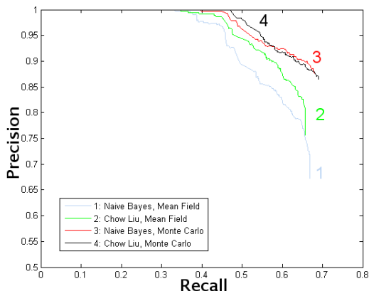
Figure 4. Precision-Recall curves for the four variant algorithms on the New College data set. Notice the scale. All results include the location prior which allows evidence to accumulate through a sequence of observations.
