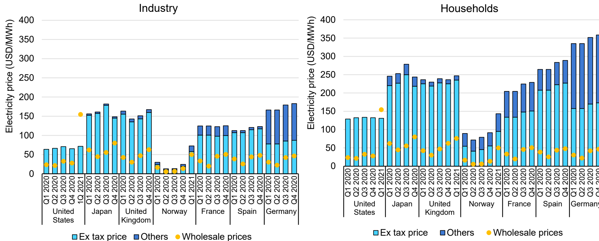
Quarterly end-user electricity prices in selected markets
