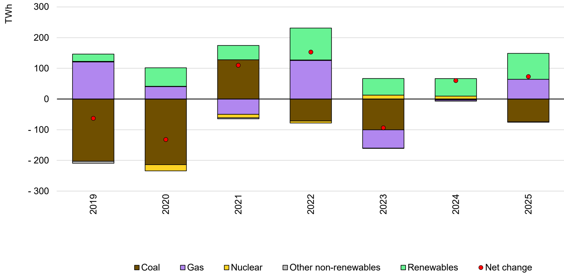
Year-on-year change in electricity generation in the United States, 2019-2025
