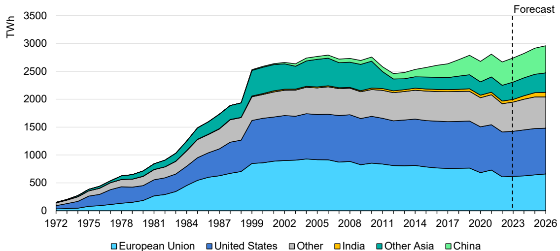
Evolution of nuclear power generation by region, 1972-2026
