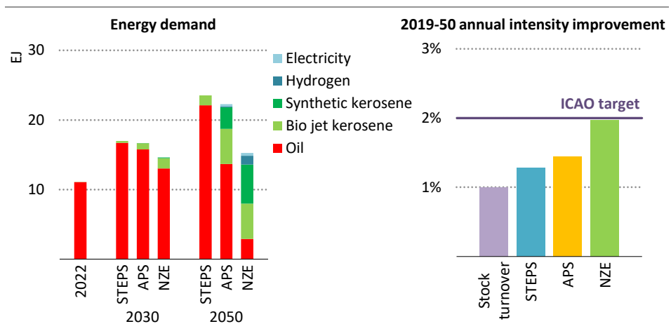
Figure 3.9 ▶ Energy demand in aviation by fuel and scenario, 2022-2050, and annual fuel intensity improvement rate, 2019-2050
