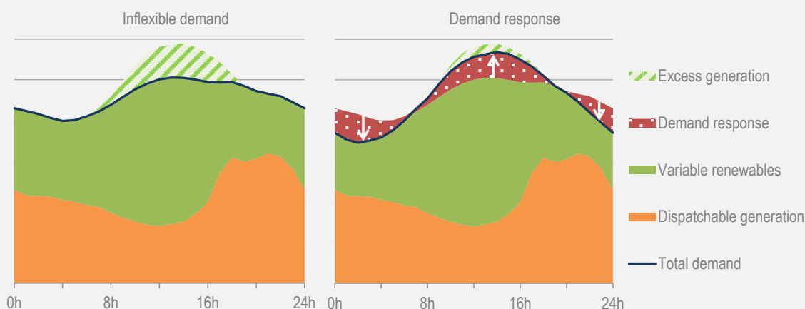
Figure 4.6 Impact of demand response on the daily load curve
