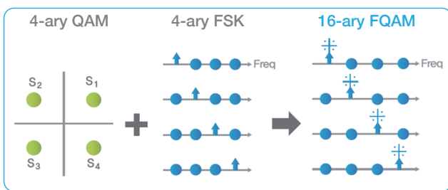
Figure 18 Example of 16-ary FQAM
