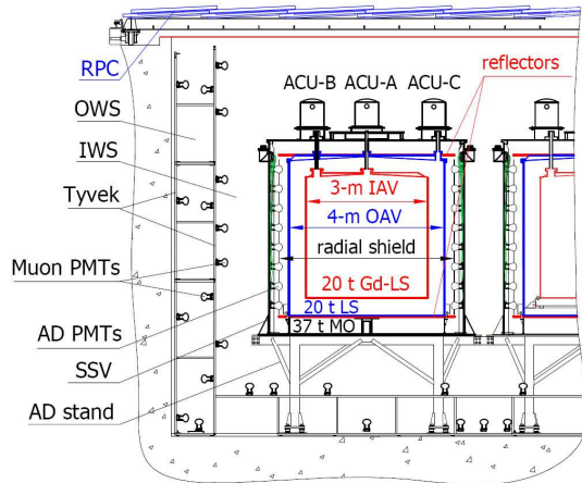
FIG. 2. Schematic diagram of the Daya Bay detectors.
