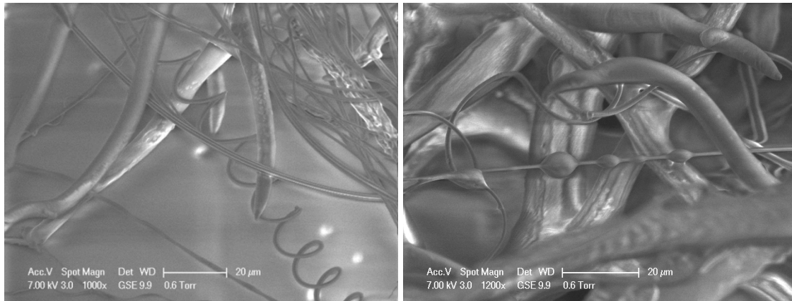
Figure 1 Environmental scanning electron micrographs of spider silk fibers illustrating the different structures present including spring-like motifs (left) and droplets of glue (right).
