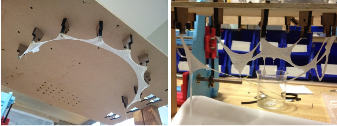
Figure 5 Images of nylon 6,6 membranes created by turning and dipping a shallow container of nylon prepolymer onto adjacent pegs (left) and by formulating the nylon prepolymer solution using 50% bubble solution (right).
